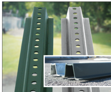
8' Steel Green & Galvanized Posts (2#/ft.) 3/8" Holes Drilled Even Inch
