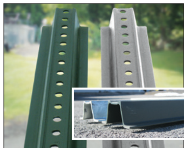
8' Steel Green & Galvanized Posts (2#/ft.) 3/8" Holes Drilled Even Inch Available in 6', 7' and 8'
